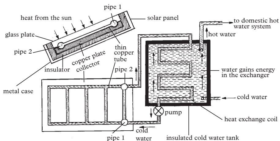
Fig. 9.17: Solar heating
