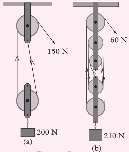
Fig. 6.23: Pulley system
