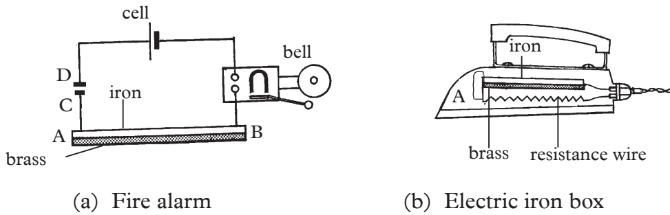
Fig. 9.26: Electric appliances with thermostat
