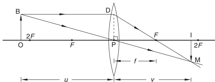
Fig. 2.29: Lens formula
