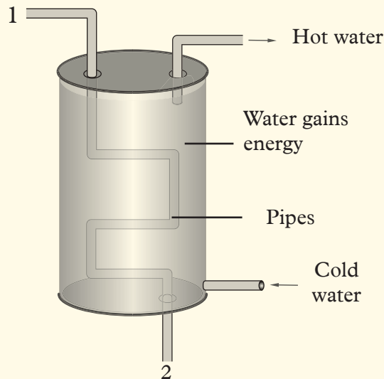
Fig. 5.31: Heat exchanger
