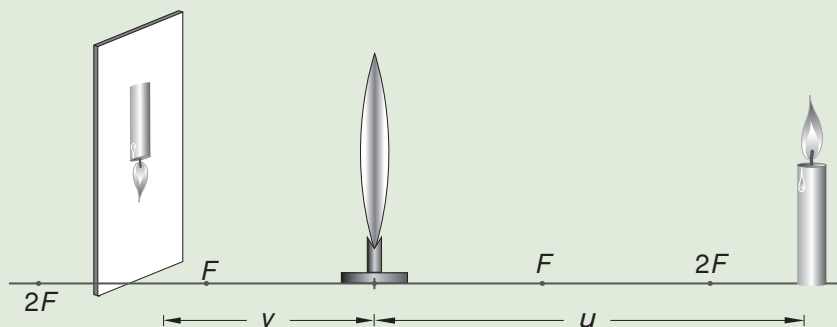
Fig. 2.14: Image formation by a far object
