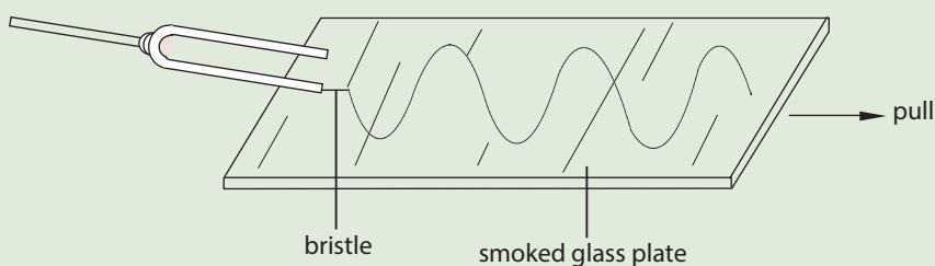
Fig. 8.3: Vibrating tuning fork on a glass plate.
