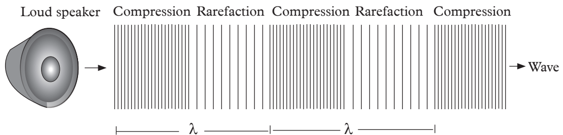
Fig. 7.13: shows a longitudinal plane waves
