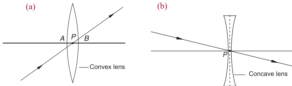
Fig. 2.13: Optical centre of a convex and concave lenses
