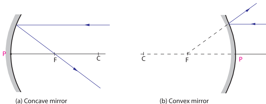
Fig. 1.18: Rays parallel and close to principle axis
