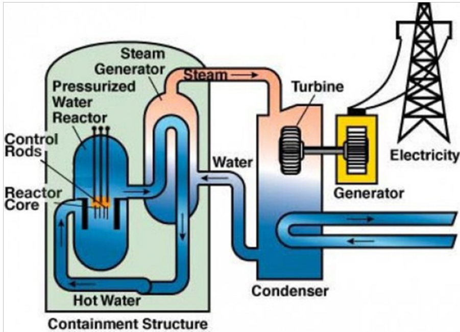
Fig 5.13: Nuclear plant
