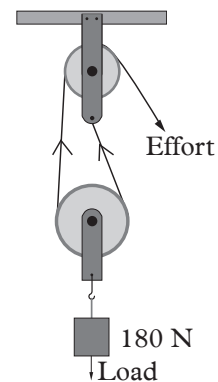
Fig. 6.25: Pulleys system
