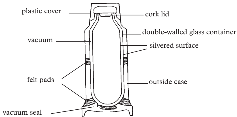
Fig. 9.12: Vacuum flask
