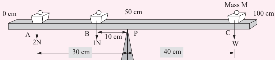
Fig. 3.10: Principle of moment
