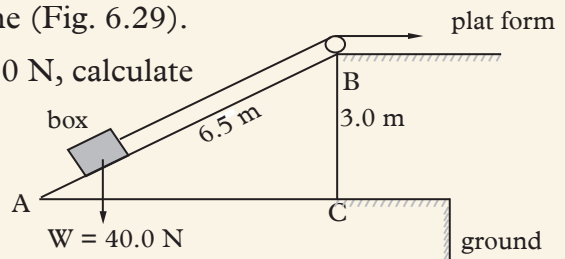
Fig. 6.29: A crane
