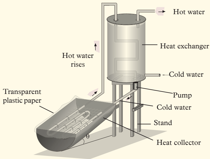
Fig 5.33: Solar heater
