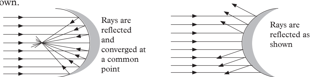
Fig 1.2: Reflection of light at curved surfaces
