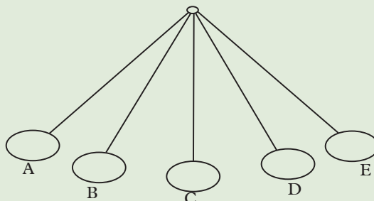
Fig. 5.24: A swinging pendulum
