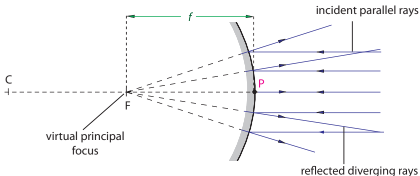
Fig. 1.7: Virtual principal focus
