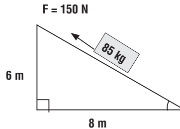
Fig. 5.7: Work done on an inclined
