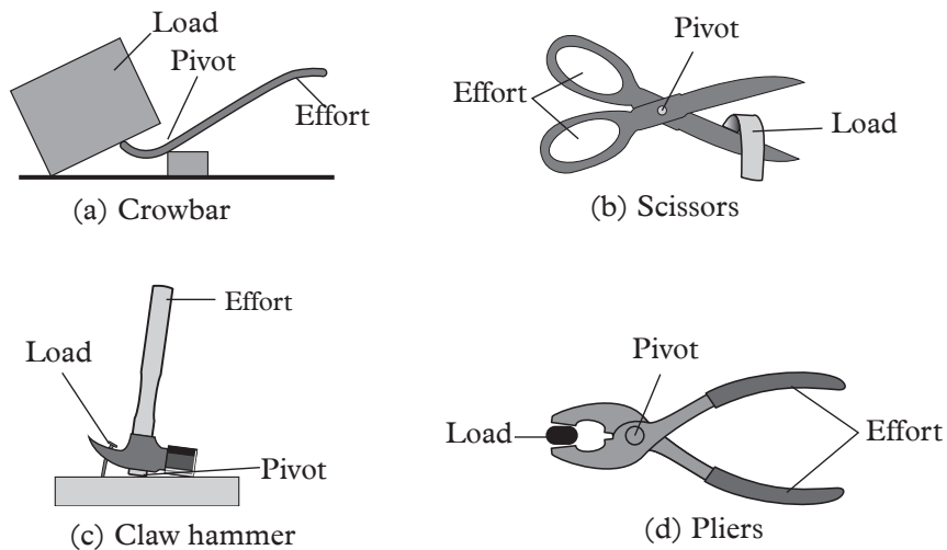
Fig. 6.2: Pivot between the load and the effort
