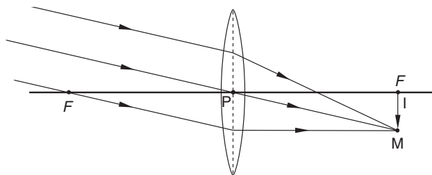
Fig. 2.18: Object OB at infinity
