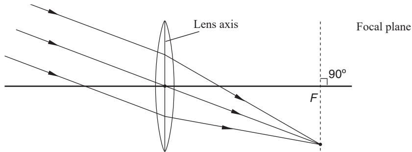
Fig. 2.12: Focal plane of a convex lens
