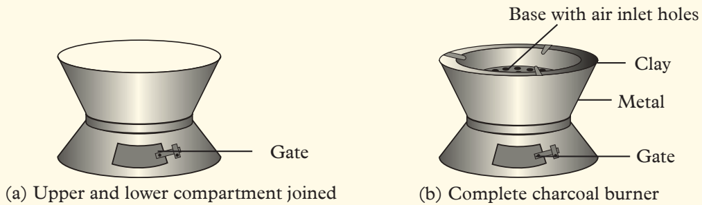
Fig. 5.29(a): Upper and lower compartments joined to make a complete charcoal burner
