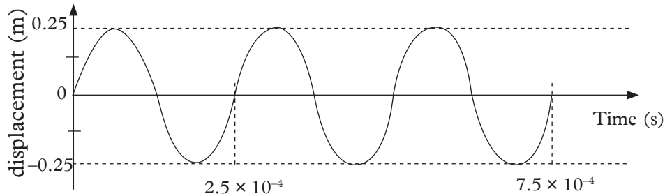
Fig. 7.21: Displacement - time graph
