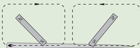
Fig. 10.20: Making a magnet with consequent poles
