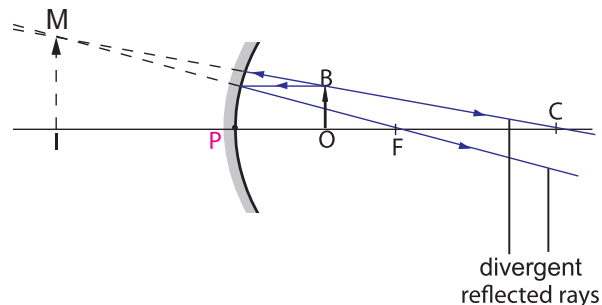
Fig. 1.27: Object between F and P
