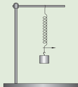
Fig. 7.5: Hanged spiral spring
