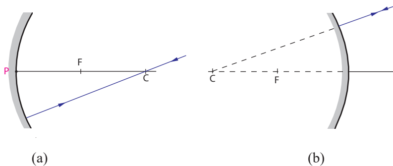
Fig. 1.20: Ray through the centre of curvature
