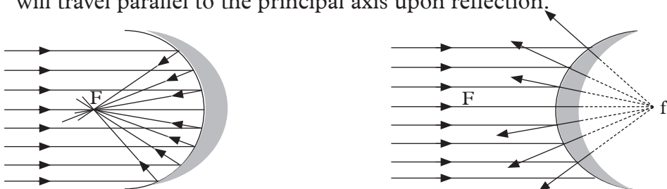
Fig. 1.4: Reflection of light at curved mirrors
