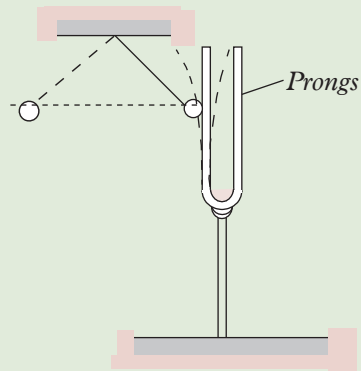
Fig. 8.2: Vibrating tuning fork displaces a pith ball.
