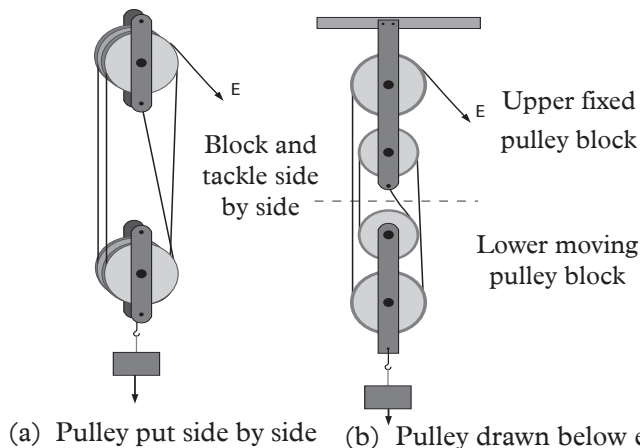
Fig. 6.19: Block and tackle systems.
