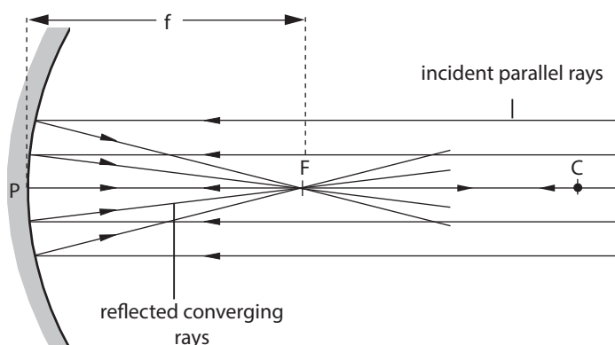
Fig. 1.6: Real principal focus
