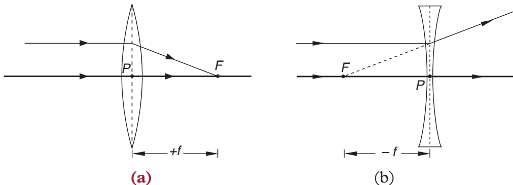
Fig. 2.30: Real and virtual focal lengths of lenses
