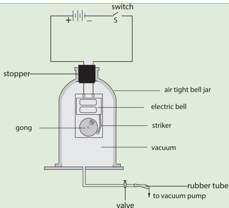
Fig. 8.9: Electric bell
