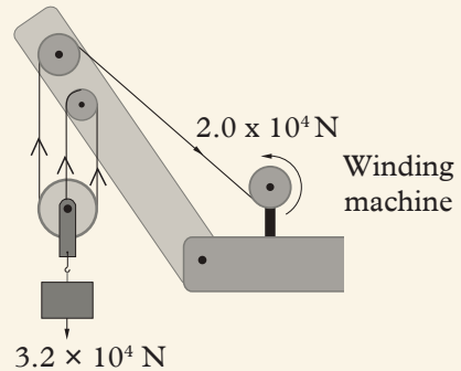
Fig. 6.32: A winding crane
